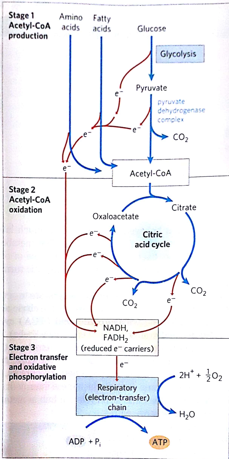
FIGURE 16-1 Catabolism of proteins, fats, and carbohydrates in the three stages of cellular respiration. Stage 1: oxidation of fatty acids,
