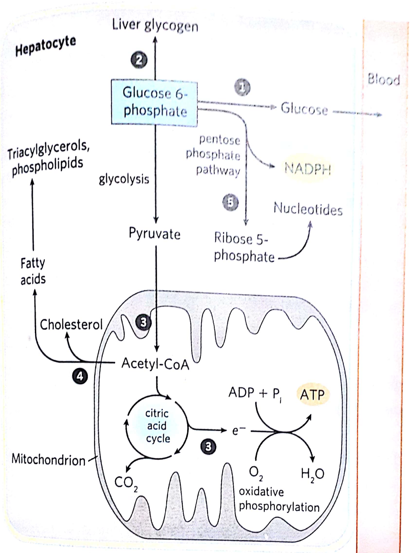
FIGURE 23-12 Metabolic pathways for glucose 6-phosphate in the liver. Here and in Figure 23-11
