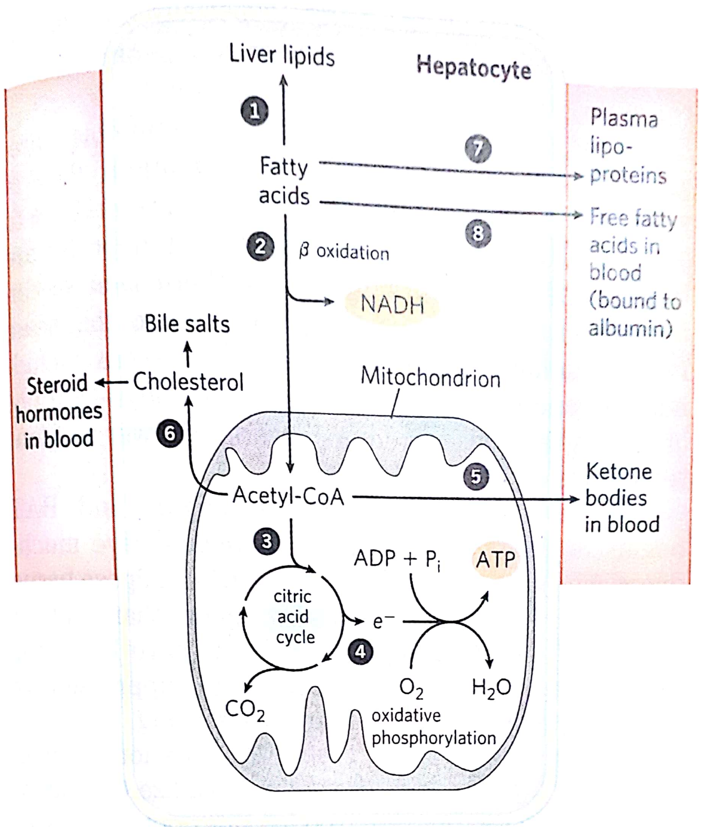
FIGURE 23-14 Metabolism of fatty acids in the liver.
