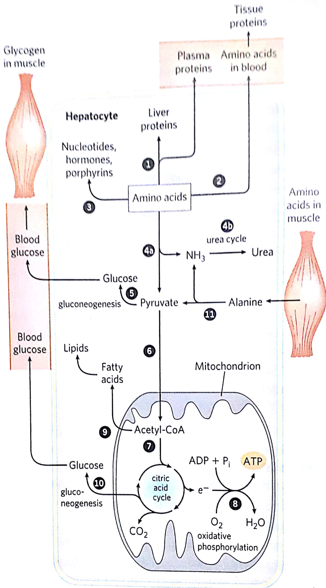
FIGURE 23-13 Metabolism of amino acids in the liver.
