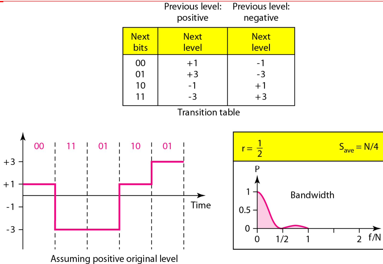
Figure 4.10 Multilevel: 2B1Q scheme
