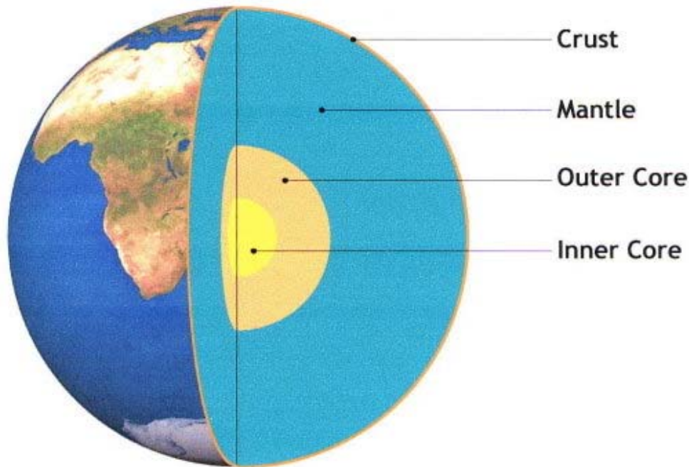
Figure 1. The concentric layers of the Earth
