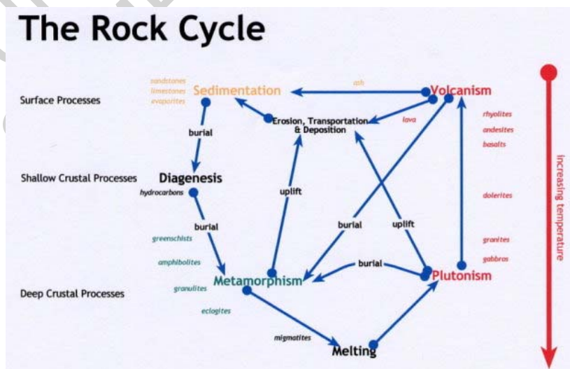
Figure 2. The rock cycle (rocks named are discussed in the text)
